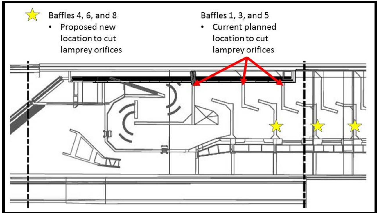
Figure 1. Bonneville Bradford Island fish ladder exit control section. Red arrows show the current location of lamprey orifices to be cut during the following in-water work period (17/18). Yellow stars are proposed new locations replacing currently planned locations.
